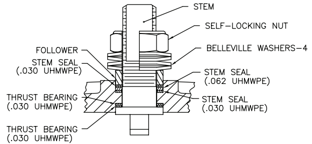
Oxygen Service Valves with UHMWPE “U” Seats Automated Valve Shown
